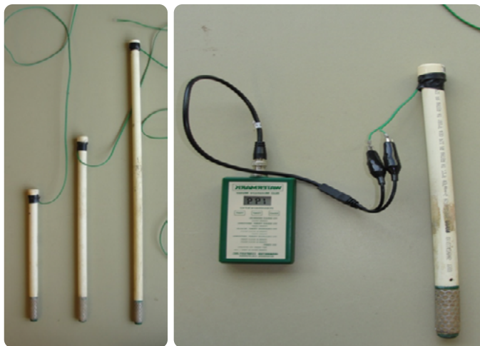
Figure 1. Manual reader and Watermark™ sensors installed on CPVC pipe for installation and different depths.
